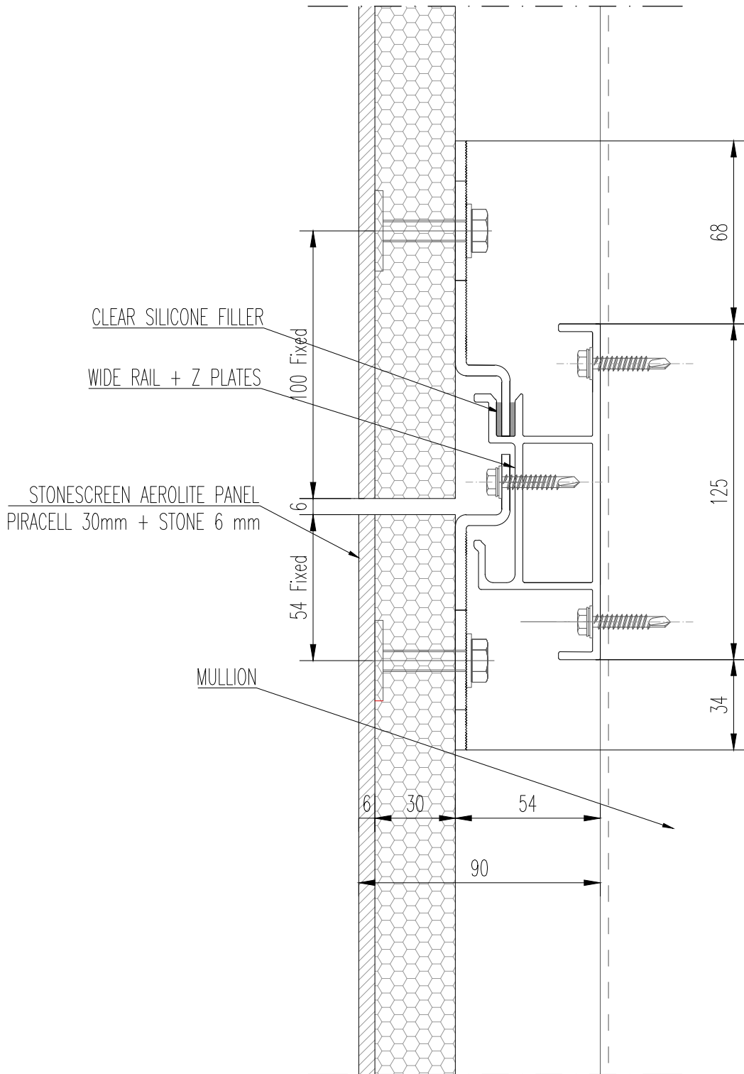
S3 Wide Support Rail + Z Plates Scale 1:2 @A4
