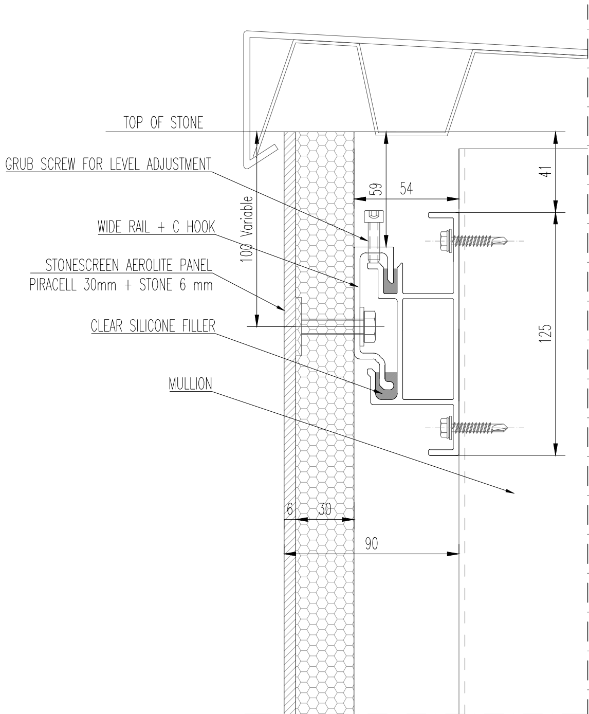
S2 Wide Support Rail + C Hook Scale 1:2 @A4
