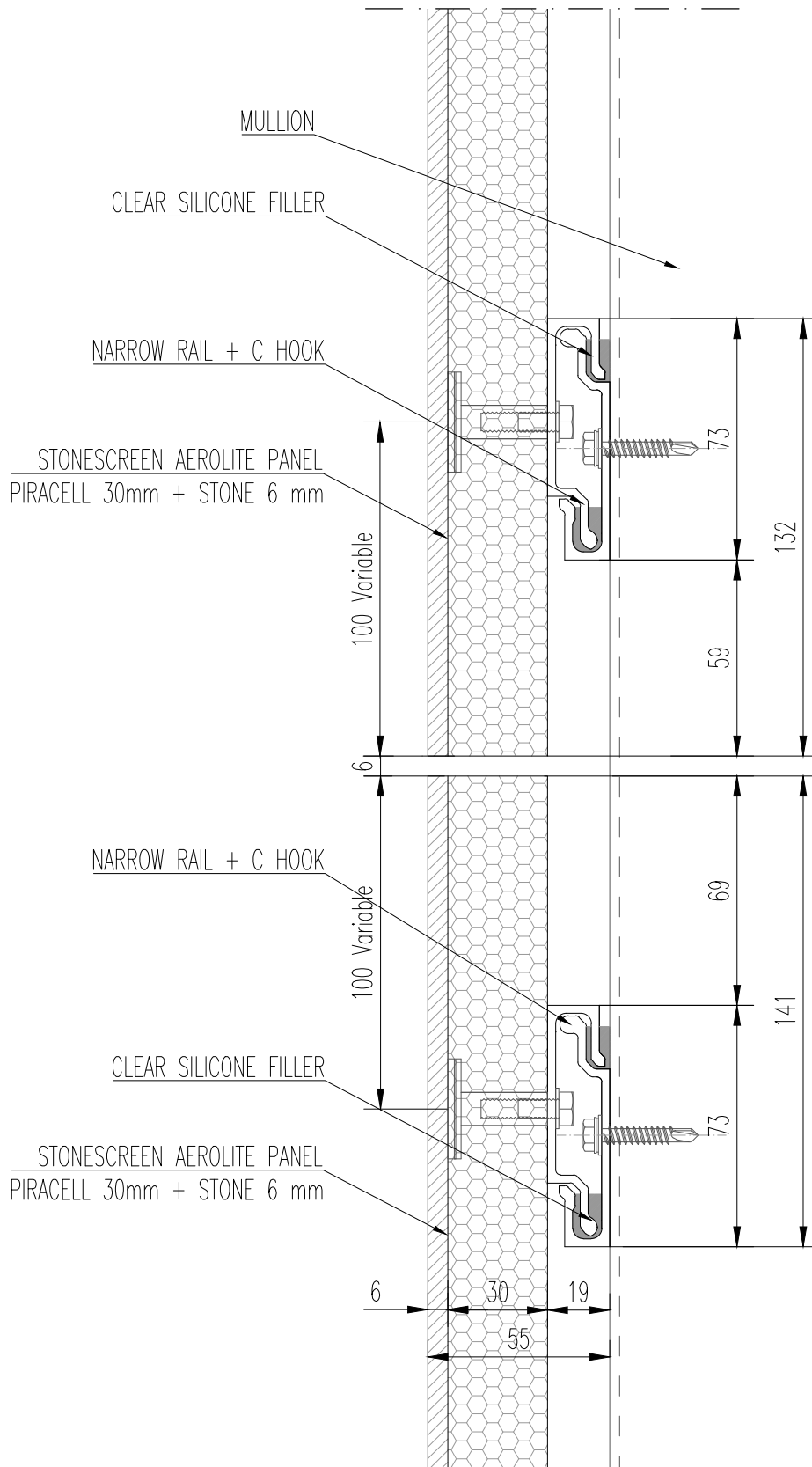
S1 Narrow Support Rail Scale 1:2 @A4
