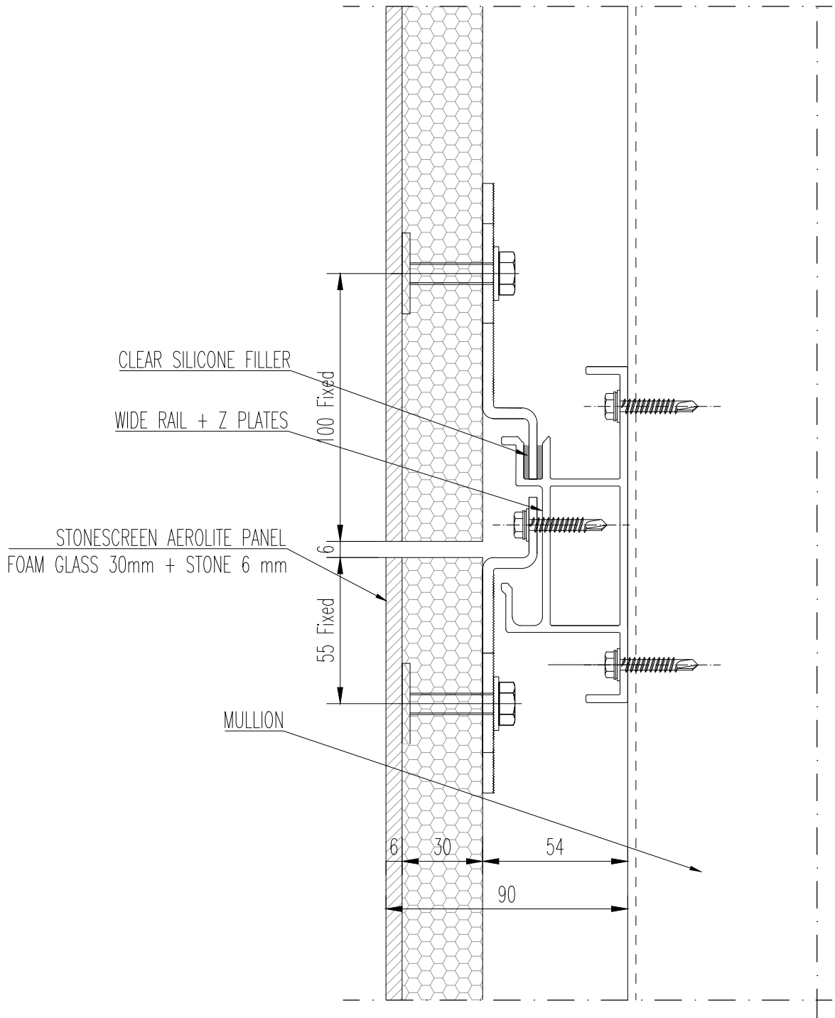
S4 Wide Support Rail + Z Plates
