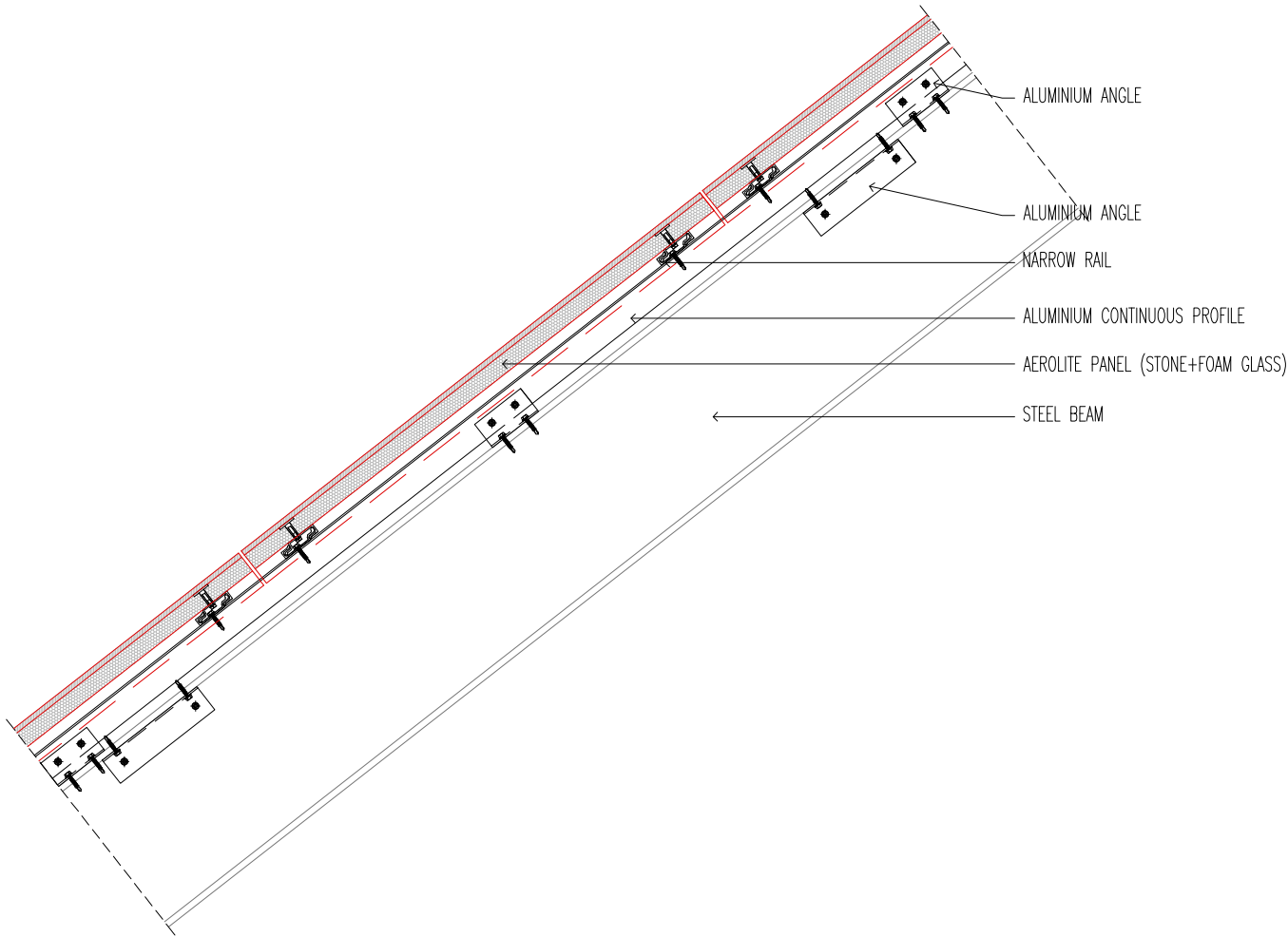
1 COPING DETAIL_GABLE TD04
