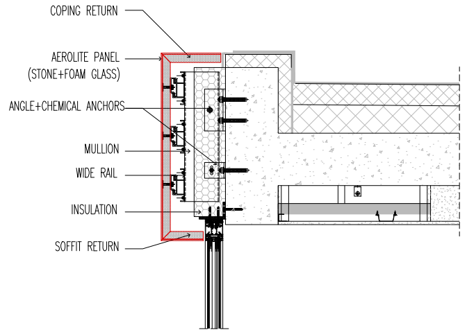
2 TOP ROOF DETAIL_CONCRETE SLABS+WINDOW TD02
