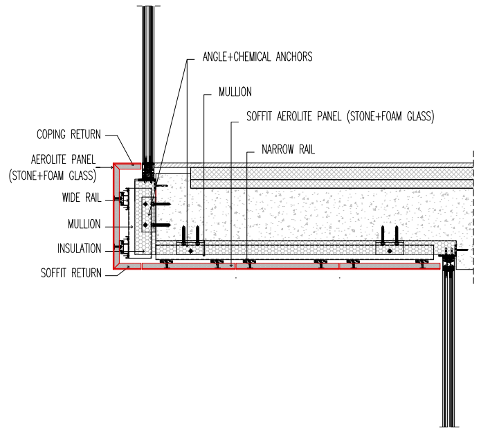
3 DETAIL_CONCRETE SLABS+WINDOW TD02
