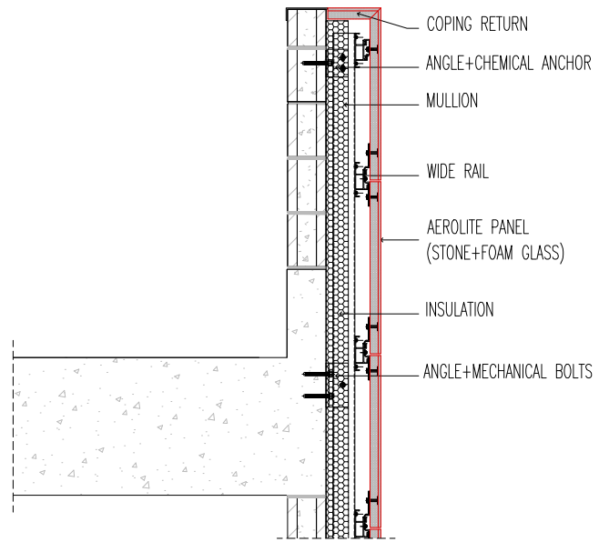
2 TOP ROOF DETAIL_CONCRETE SLABS+BLOCKWORK TD01
