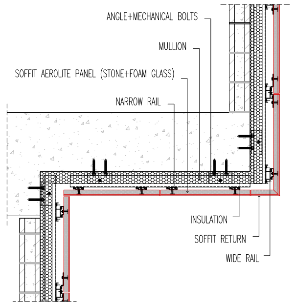
3 DETAIL_CONCRETE SLABS+BLOCKWORK TD01
